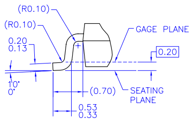
DETAIL A SCALE: 30:1
